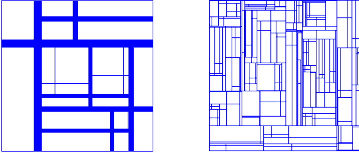
FIGURE 1: Two splittings of [0, 1]^2 with 8 (left) and 100 (right) points.
