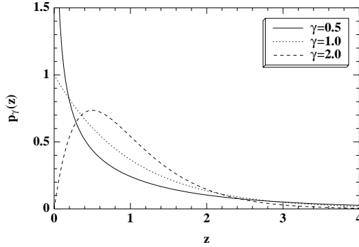
FIG. 3. Probability density of the sizes of the attraction basins under H^\gamma for different \gamma .
