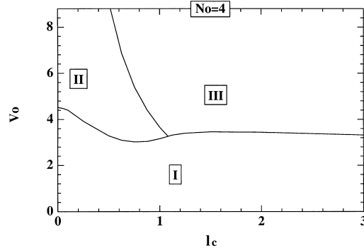
Fig. 3. The three possible regimes for an incoming soliton with mass N_0 = 4 as a function of the initial velocity V_0 and the correlation length l_c (the correlation function is assumed to have Gaussian shape). Region I corresponds to an almost constant mass and a decaying velocity. Region II corresponds to an almost constant velocity and an exponentially decaying mass. Region III corresponds to an almost constant velocity and a L^{-1/2} -decaying mass. If V_0 \gg 1 , then the boundary between regions II and III lies about l_c \sim 2\sqrt{2}\sqrt{\ln(V_0)}/V_0 . If l_c \gg 1 , then the boundary between regions I and III lies about V_0 \sim 3.3 .
