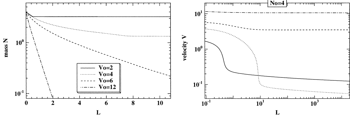
Fig. 1. Coefficients of the transmitted soliton, with the initial mass N_0 = 4 and different initial velocities. Here l_c = 0.1 and \sigma^2 = 1/(2\sqrt{\pi}) .
