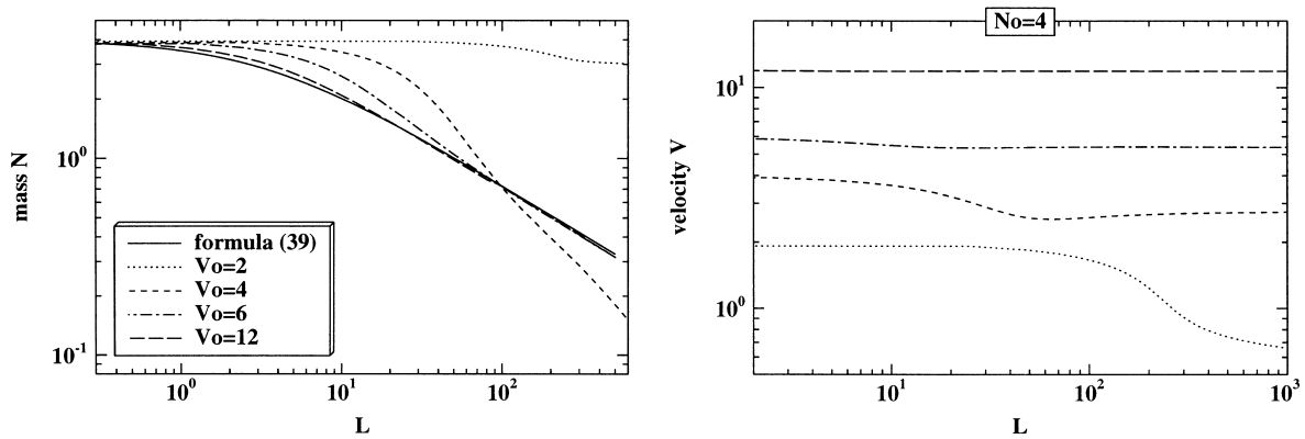
Fig. 2. Coefficients of the transmitted soliton, with the initial mass N_0 = 4 and different initial velocities. Here l_c = 2 and \sigma^2 = 1/(2\sqrt{\pi}) .
