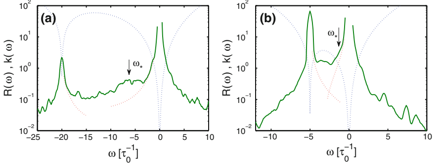
Figure 5. Applicability criterion of the wave turbulence theory, \mathcal{R}(\omega) = k_{nl}(\omega)/k(\omega) \ll 1 , for two cases considered in Figure 2: a \alpha=0.05 , b \alpha=0.2 . The function \mathcal{R}(\omega) is plotted in logarithmic scale, it has been obtained by averaging the NLS spectrum from z=2,500 to z=2,550 (over 50 realizations, \sigma=1 ). The dashed blue line shows the dispersion relation |k(\omega)| , the arrows indicate the location of the zero-dispersion frequency \omega_* (color figure online).
