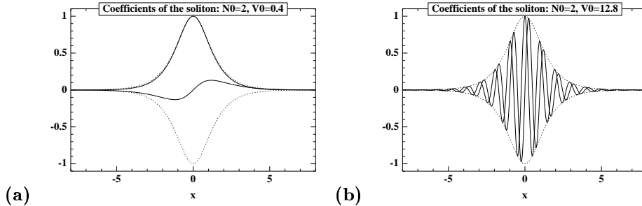
Fig. 3. Solitons at time t = 0 . The dashed lines represent the envelops of the solitons, while the solid lines represent the real and imaginary parts. Picture a: N_0 = 2 , V_0 = 0.4 . Picture b: N_0 = 2 , V_0 = 12.8 .
