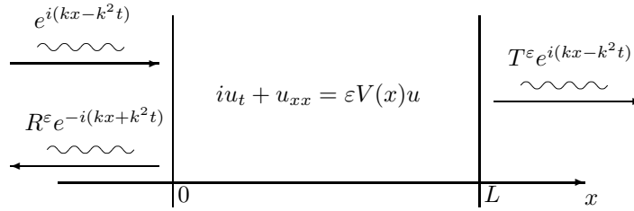
Fig. 1. Scattering of a monochromatic pulse.
